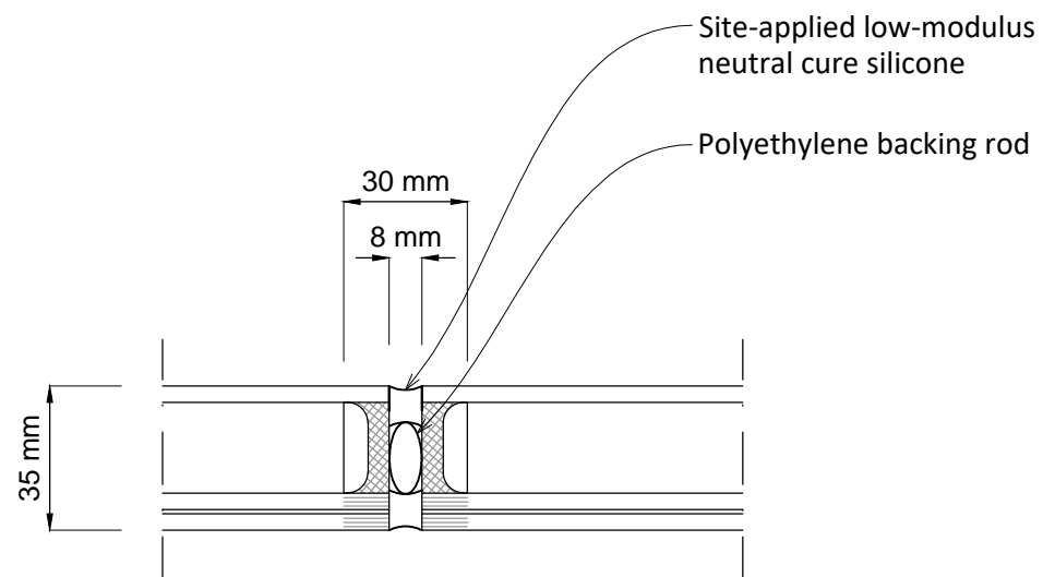
Detail A through section a-a'
