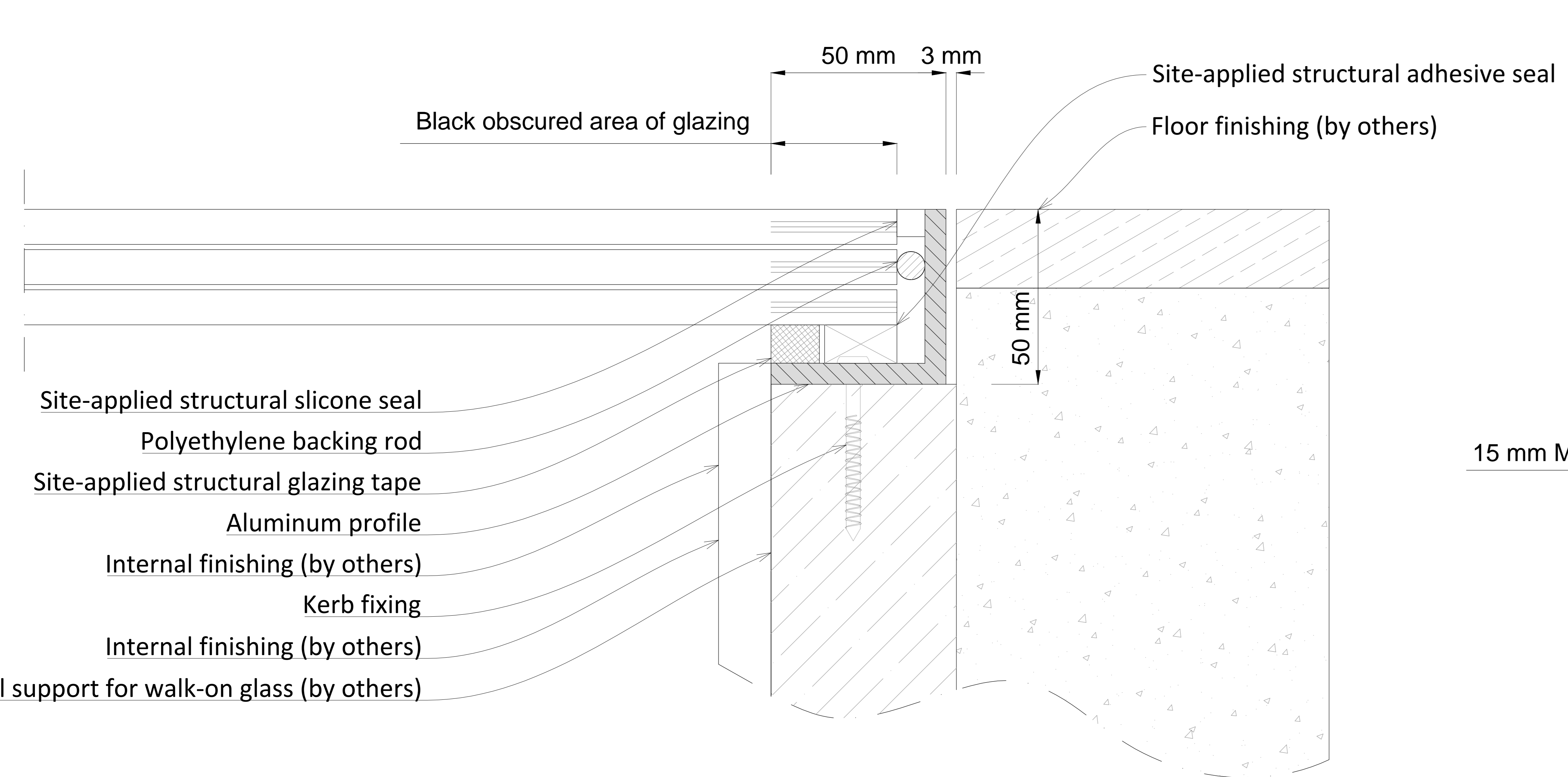
Detail A through section a-a'
