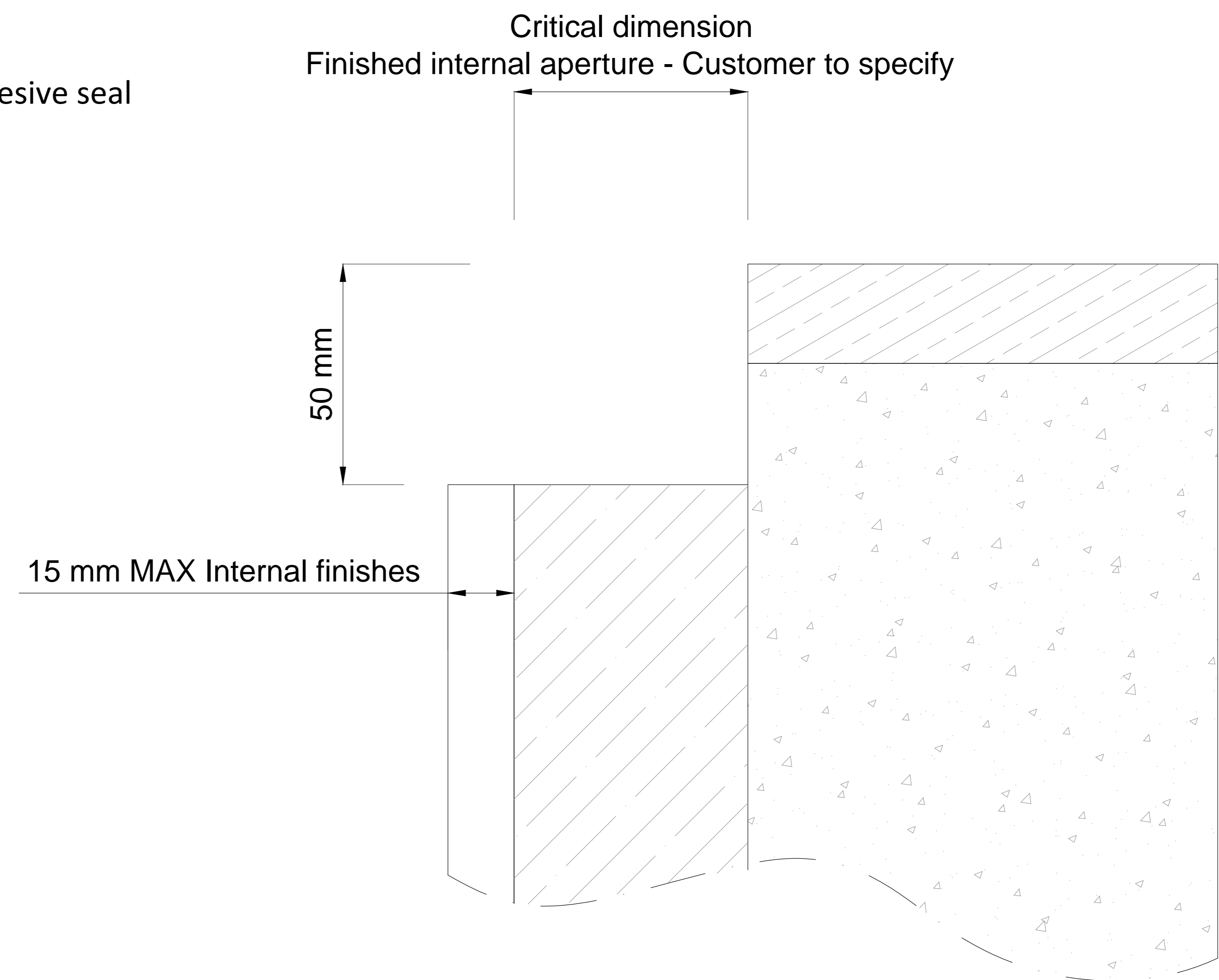
Kerb Detail A through section a-a'
